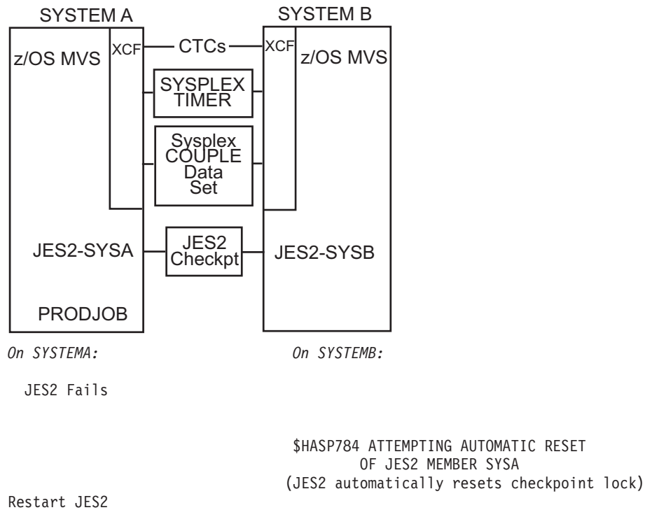
Figure 51. Sysplex with the AUTOEMEM Option Enabled, a JES2 Failure (Coupling Facility)
