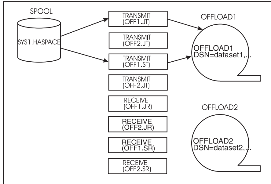
Figure 36. Offload Initialization Statements and $$ OFFLOADn,TYPE=TRANSMIT Relation
