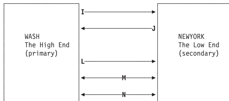
Figure 75. Two Path Manager Nodes Signon Protocol
