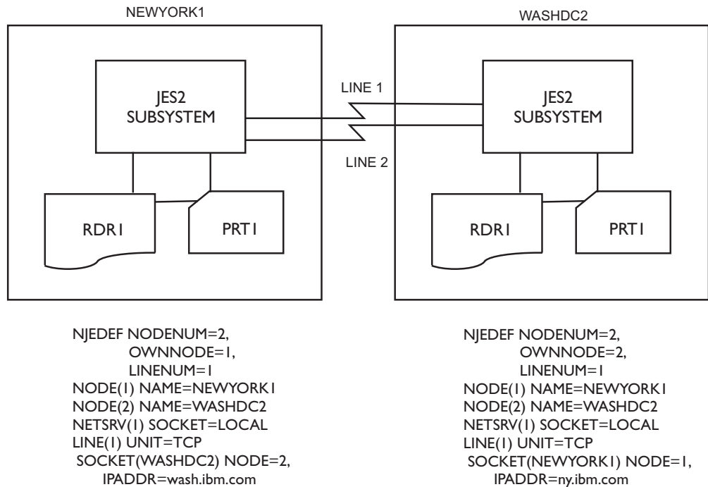
Figure 68. Basic TCP/IP Configurations
