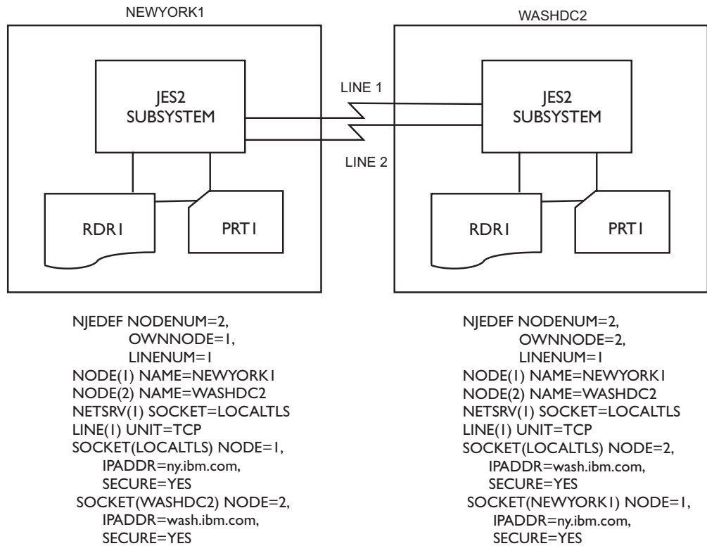
Figure 72. Secure connection from either node
