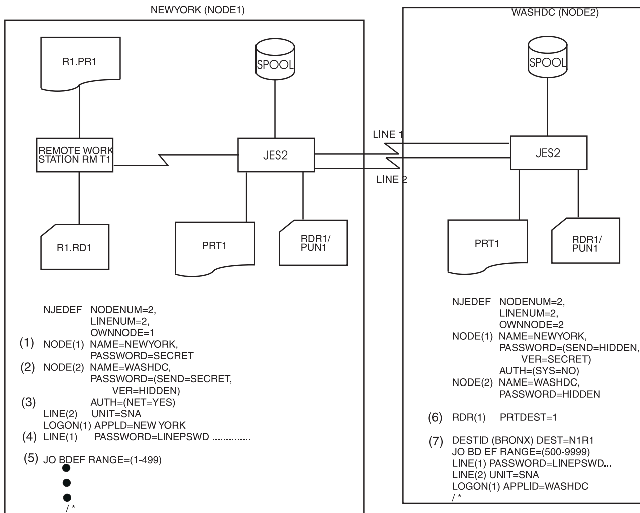
Figure 84. An Expanded Network
