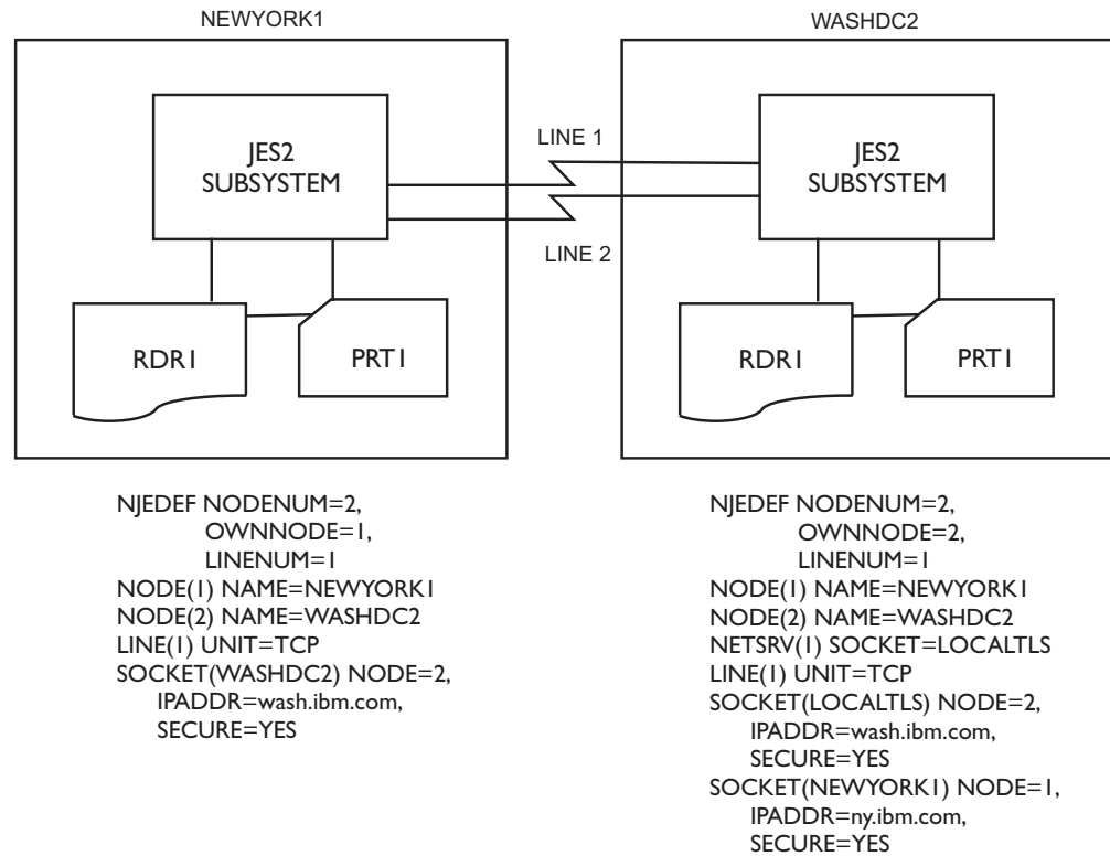
Figure 71. Secure connection from client node
