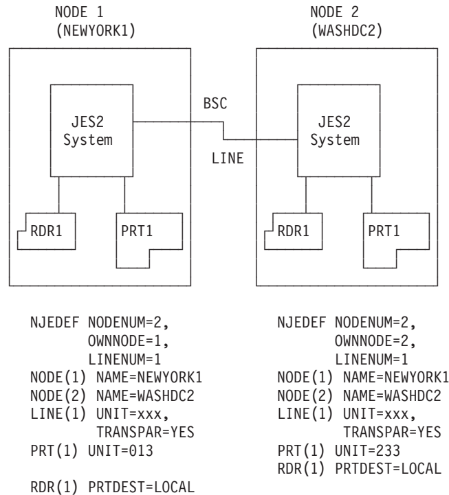
Figure 63. Minimum NJE Configuration (BSC only)
