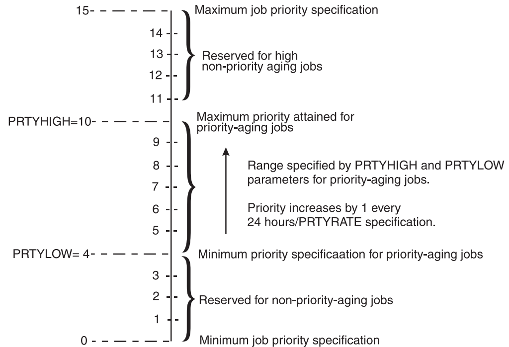
Figure 11. Example of the Interaction of Priority-Aging Parameters, PRTYHIGH= , PRTYLOW= , and PRTYRATE= on JOBDEF Statement
