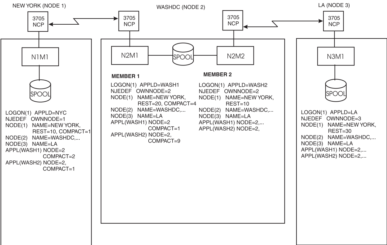
Figure 86. Multi-Access Spool Configuration (SNA)
