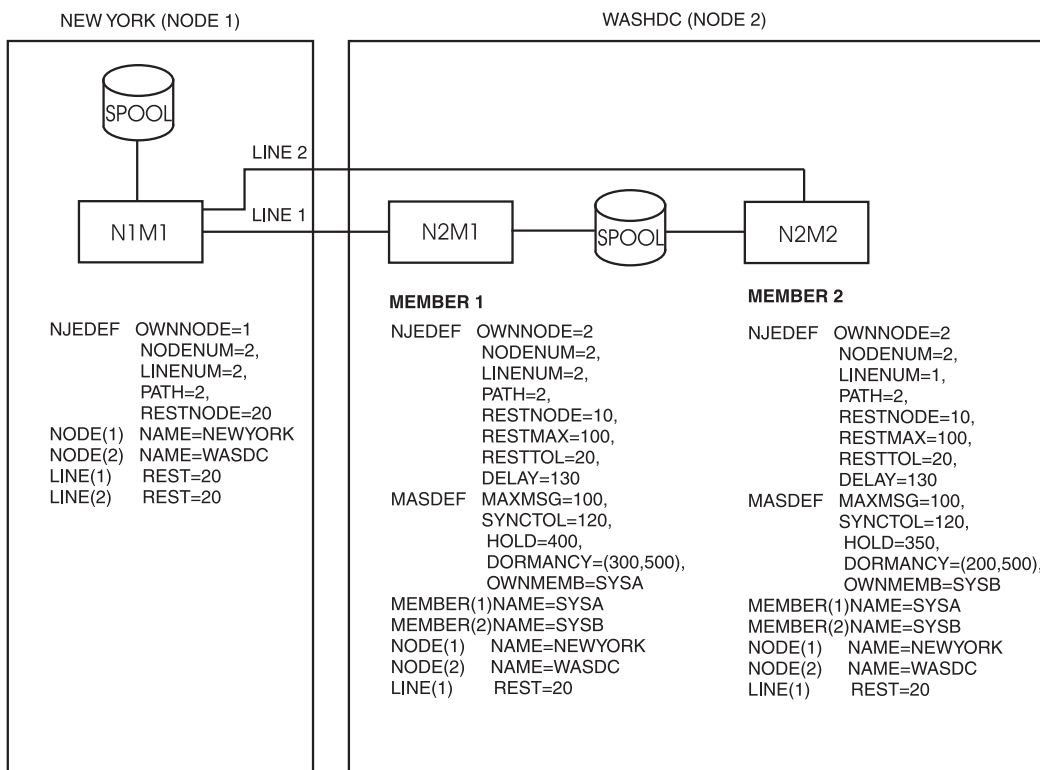
Figure 85. Multi-Access Spool Configuration (BSC)
