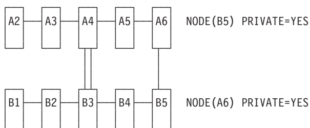
Figure 76. Two Private Nodes Across Subnets
